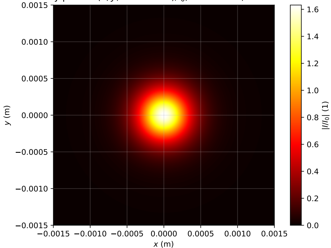
Intensity profile I(x, y, z = 2.309m)/I_0 , Pin=0.9Pcr, artificial time
